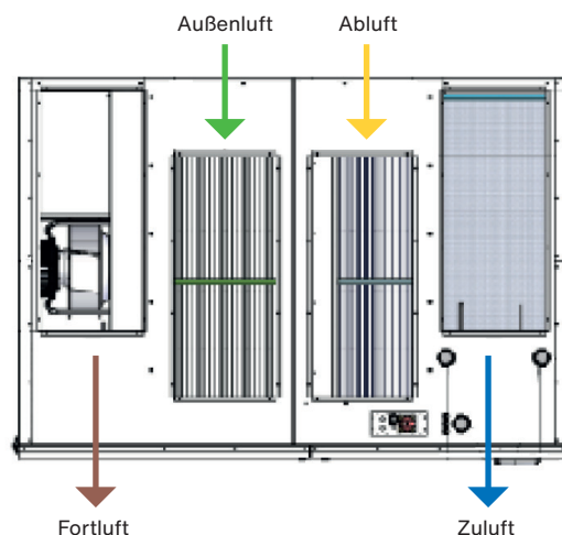
Zehnder Silvertop 52
